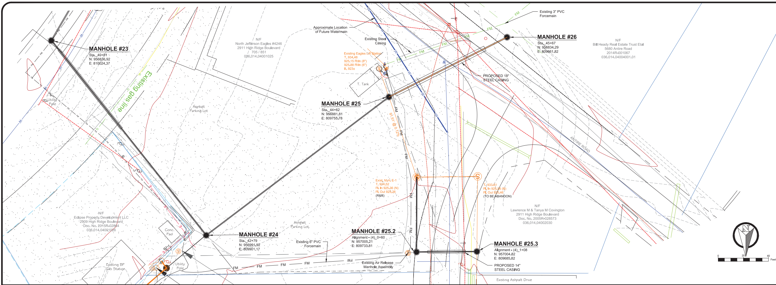
PLAN SCALE: 1:20_XREF
