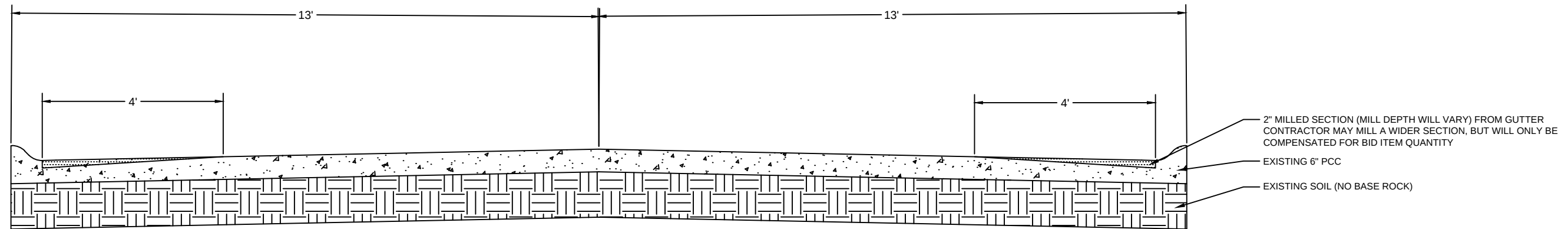
TYPICAL MILLED SECTION NOT TO SCALE. FOLLOW DIMENSIONS
