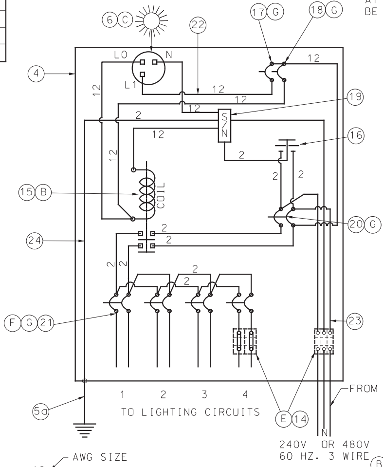
LIGHTING CONTROLLER/ DISCONNECT
