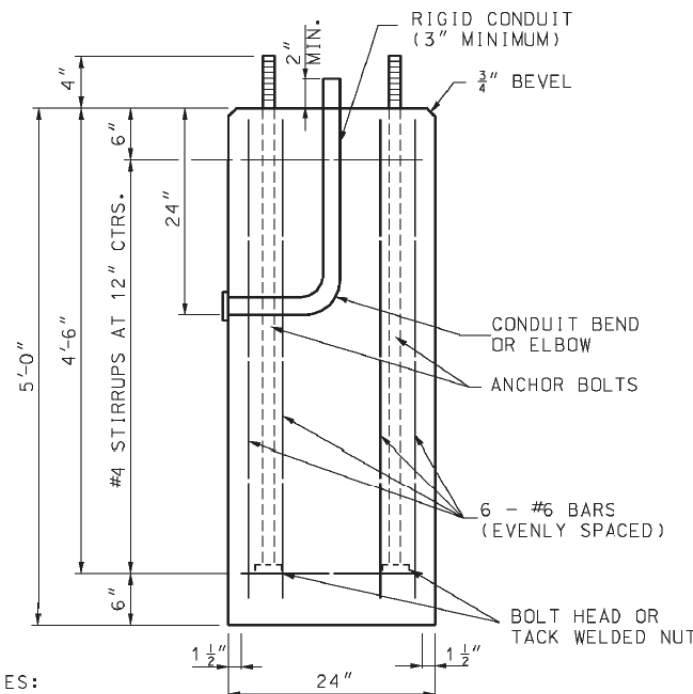
ELEVATION DETAILS OF CONCRETE FOUNDATION ③
