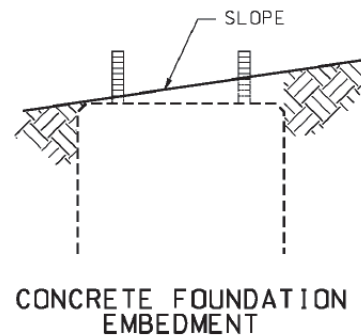
ELEVATION DETAILS OF CONCRETE FOUNDATION ③
