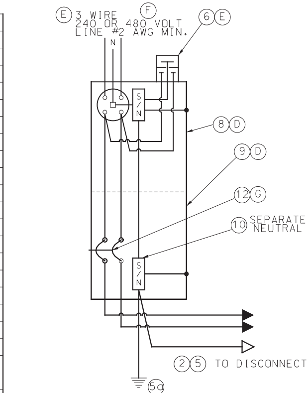
POWER SUPPLY ASSEMBLY/ METER BOX
