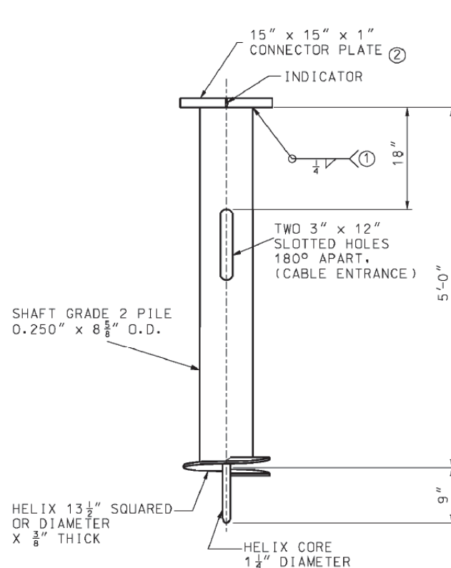
ELEVATION DETAILS OF SCREW ANCHOR FOUNDATION
