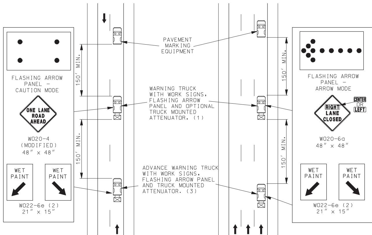
Two-Lane Undivided Highway
