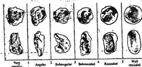
FIGURE 2: Angularity Criteria
