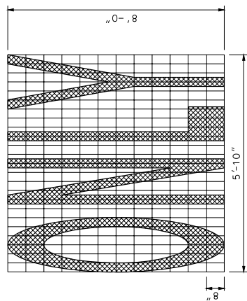
WORD MARKING ELONGATED WORD & SYMBOL
